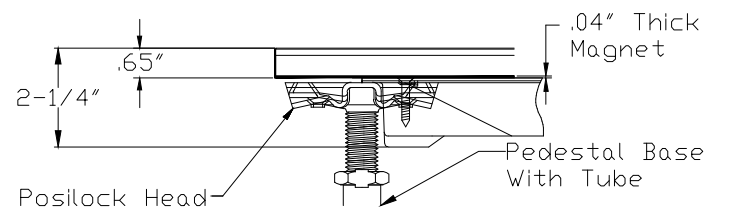
Detail A - Posilock Understructure Scale 1:2
