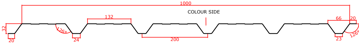
EUROCLAD EC 19-167-1000 Liner 19_2L 0.4mm Steel LINER
