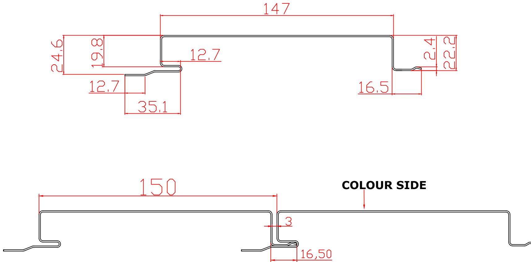
150mm Module with 3mm Gap Note: 150mm Module Opus is only available with a 3mm Gap
