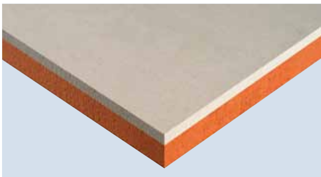
Figure 5 Super high performance Kingspan Kooltherm™ K18 Insulated Plasterboard
